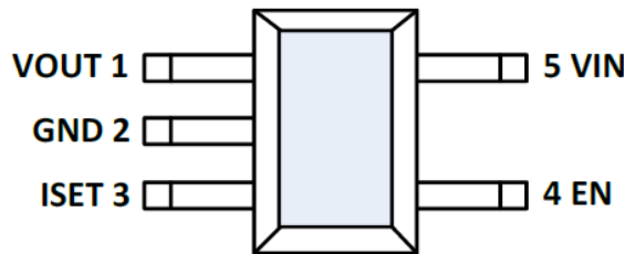
SOT23-5(Top View) Pin Configuration of EC9521
