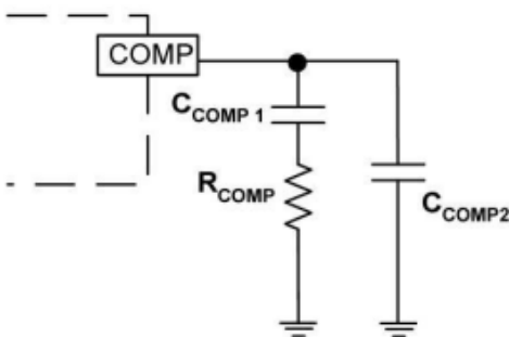
Figure 2. Stability Compensation
