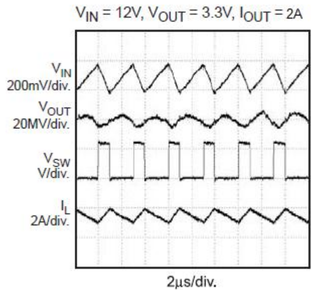
Figure 6. Steady State Test
