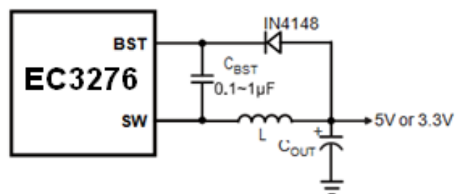
Figure14.Add Optional External Bootstrap Diode to Enhance Efficiency
