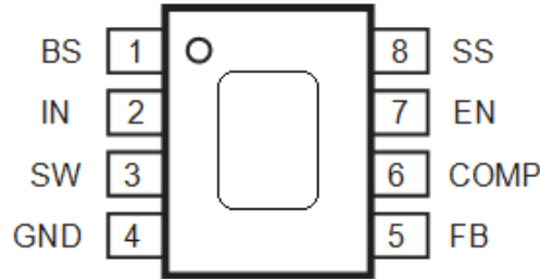
Figure 2 Pin Configuration of EC3276(Top View)
