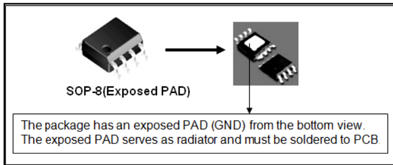
Figure 3. Package Types of EC3276
