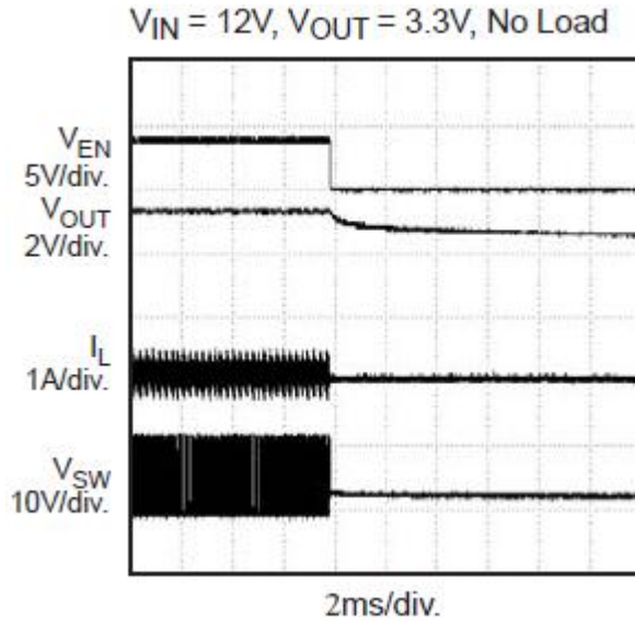
Figure 9. Shutdown through Enable
