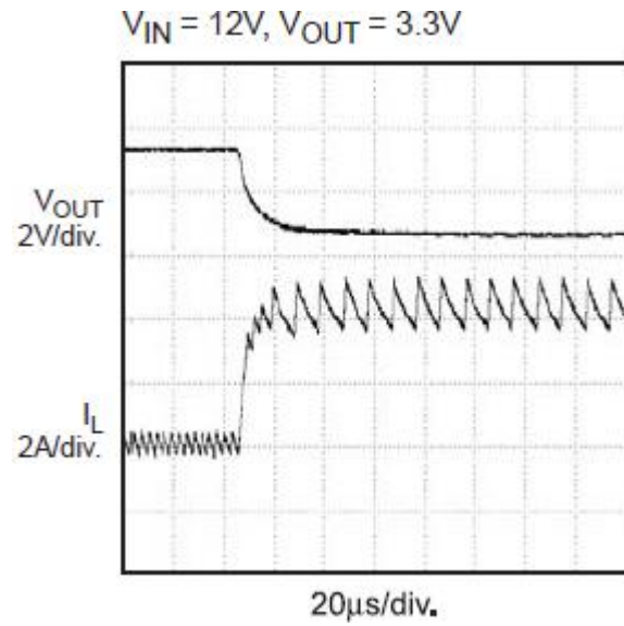
Figure 12. Short Circuit Test
