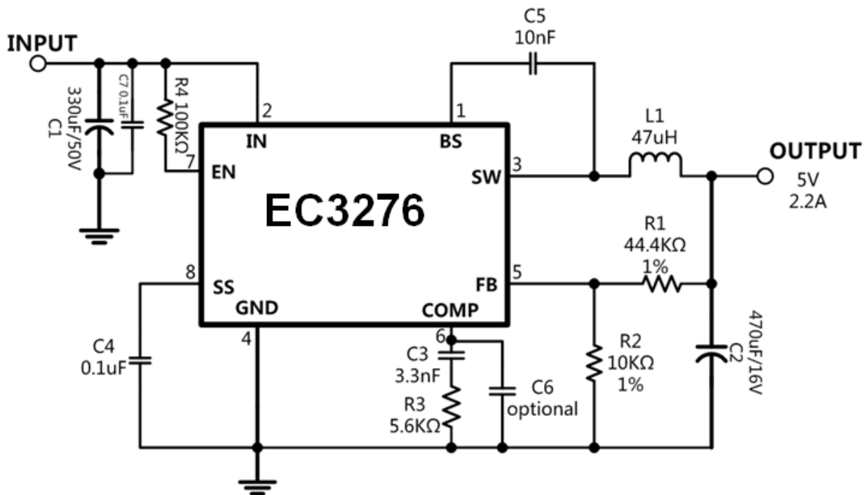
Fig1. EC3276 with 5V Output, 470μF/16V Electrolytic Output Capacitor
