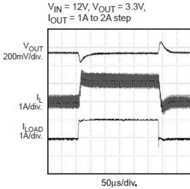
Figure 11. Load Transient Test
