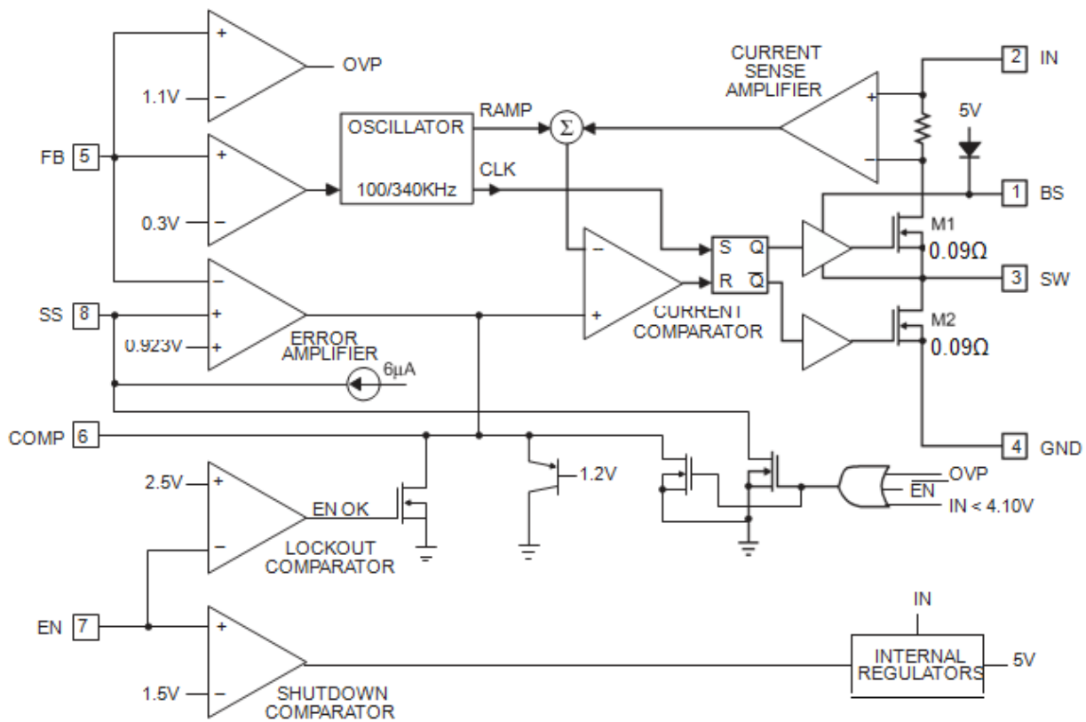
Figure 4 Function Block Diagram of EC3276
