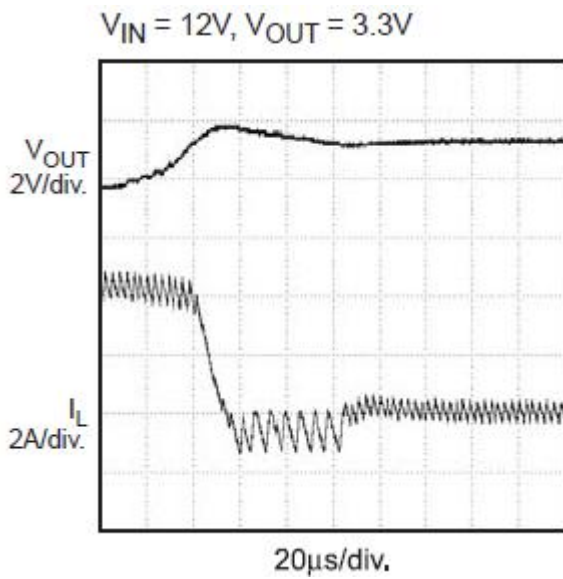
Figure 13. Short Circuit Recovery
